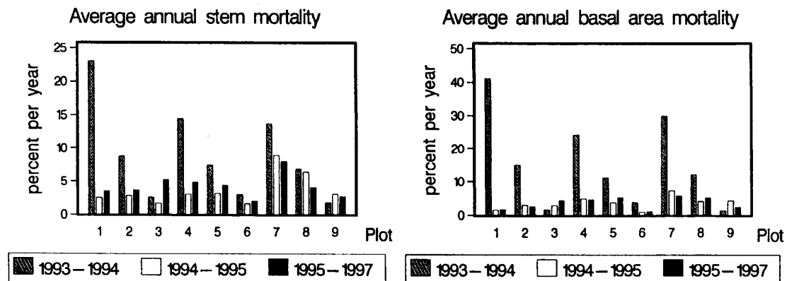
Fig. 1. Annual rates of stem and basal area mortality. Data from permanent sample plots located in high restinga (plots 1-3), low restinga (plots 4-6), and tahuampa (plots 7-9) flood plain forests at Braga-Supay and Lobillo, Peruvian Amazon. Plots 1, 4, and 7 were treated with a heavy felling, plots 2, 5, and 8 with a moderate felling, while plots 3, 6, and 9 are untreated.
