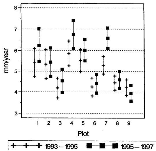
Fig. 5. Mean and 95% confidence limits for the average annual diameter increment (mm per year) of individuals \geq 10 cm DBH in permanent sample plots located in high restinga (plots 1-3), low restinga (plots 4-6), and tahuampa (plots 7-9) flood plain forests at Braga-Supay and Lobillo, Peruvian Amazon. Plots 1, 4, and 7 were treated with a heavy felling, plots 2, 5, and 8 with a moderate felling, while plots 3, 6 and 9 are untreated.
