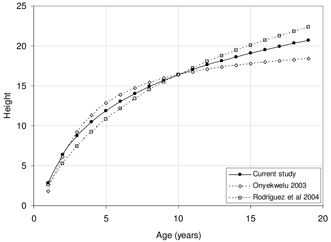
Figure 2. Comparison of Equation (1) with published site index equations for Gmelina arborea (Onyekwelu 2003, Rodríguez et al 2004)
