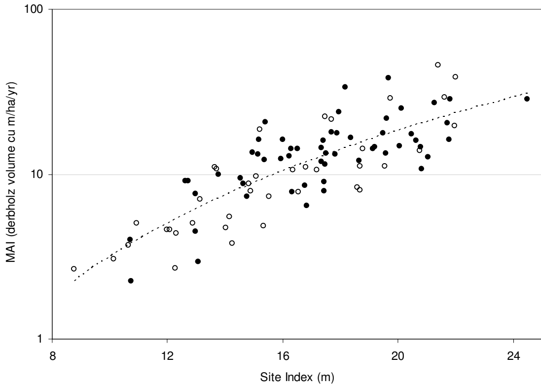
Figure 4. The relationship between site index and volume MAI
