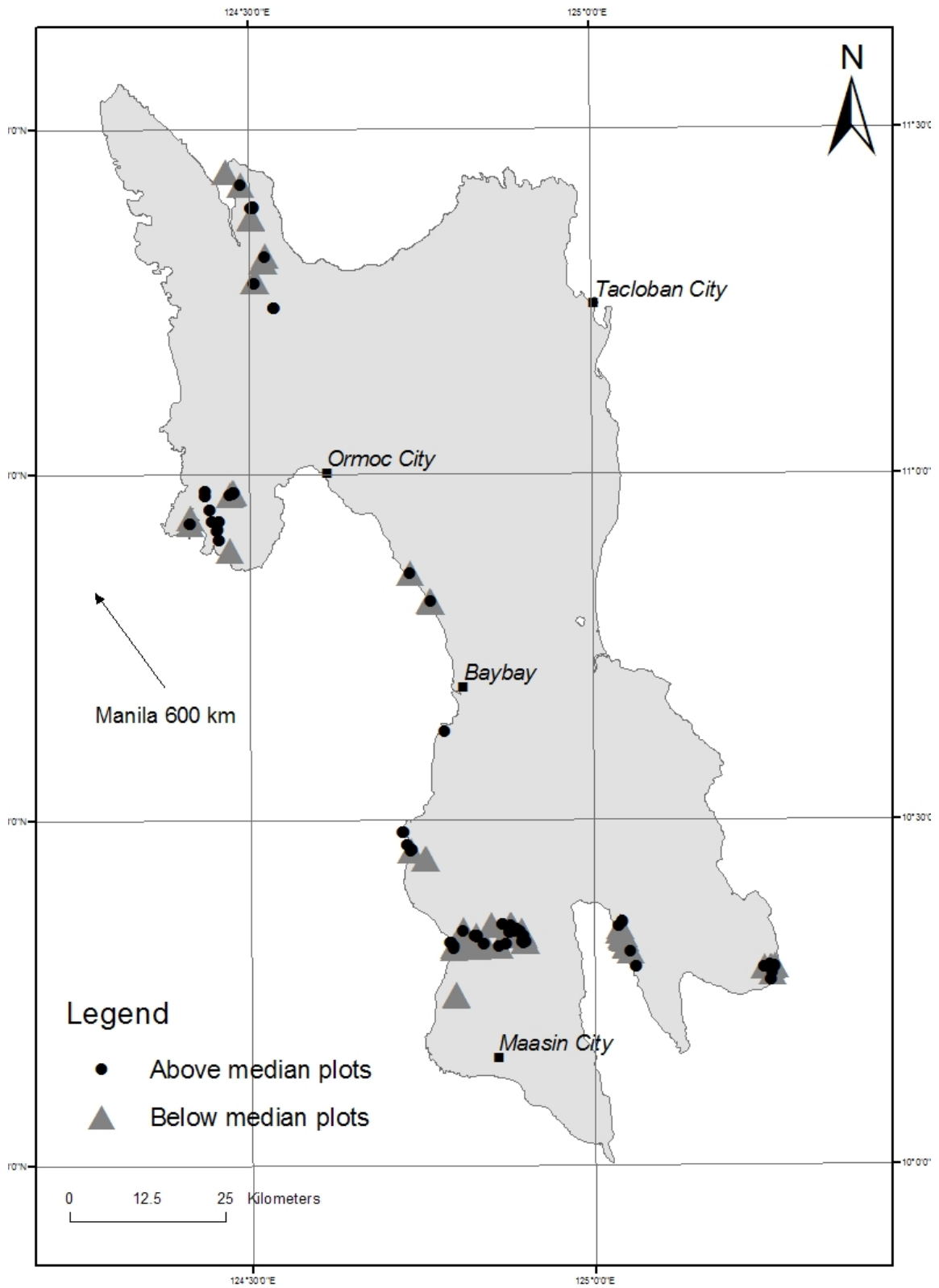
Figure 5. Geographic distribution of plots and site index on the island of Leyte, The Philippines
