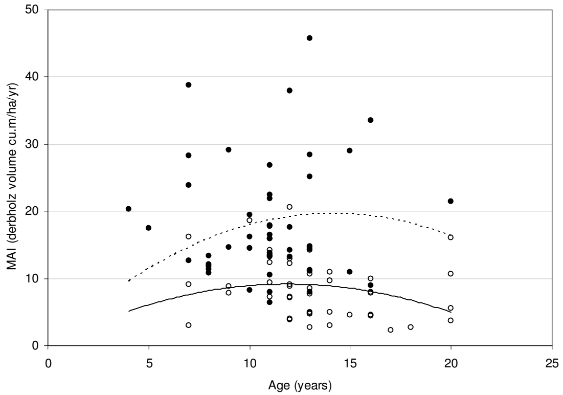
Figure 3. Mean annual volume increment (MAI) trends for above- and below-median site-index stands
