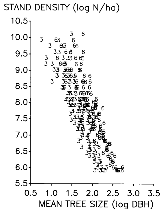
Fig. 7. Size-density diagram for clinal plots of Eucalyptus in India at 3 and 6 years of age. Each point is the mean of up to 16 replications. Notice that a good range of density and size is sampled, even after only 3 years.
