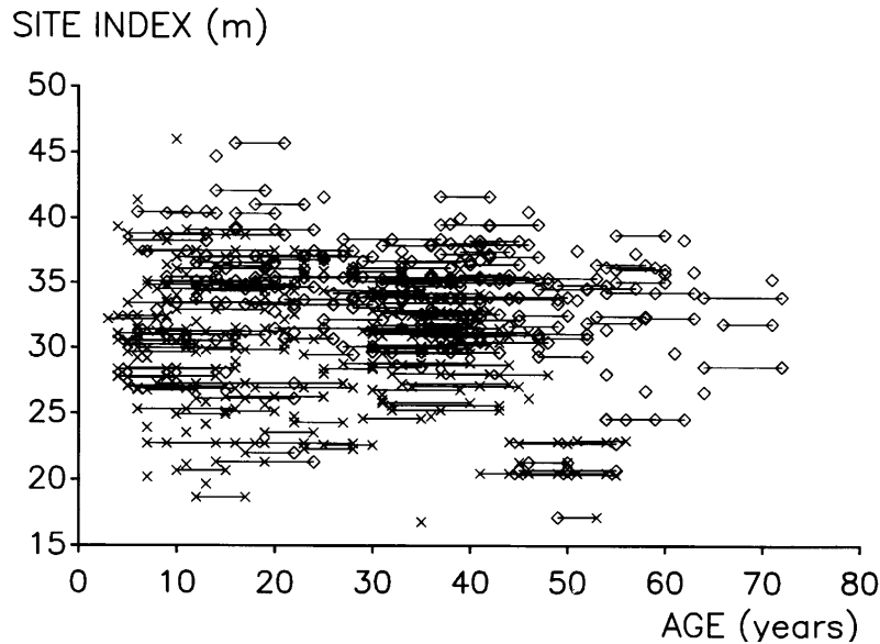
Fig. 1. Range of site index and age in Burma data. Symbols indicate plots above ( \circ ) and below ( \times ) the mean stand basal area. Lines join remeasures on the same plot. Site index (height in metres at age 80 years) is the average of all measures.
