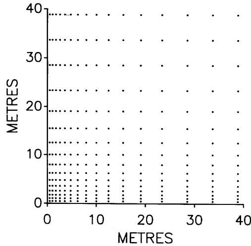
Fig. 6. Planting positions used in each block of the Adlard et al. (1992) clinal spacing experiment.
