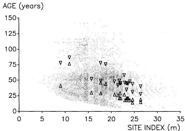
Fig. 3. Stand age vs. site index (height in metres at age 50 years). Stands are classified on site index using a computerised version of Moller (1933) to allow comparisons. Symbols indicate the FMDB (•) and the age range represented on PSPs ( \Delta - \nabla ).
