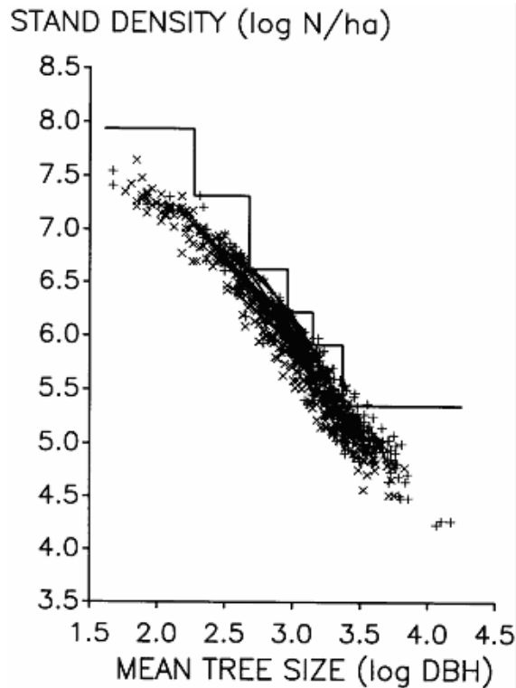
Fig. 2. Mean tree size and stand density in Burma data. Lines join remeasures on the 15 plots measured four times. The stepped line is a silvicultural prescription (Streets, 1962). Symbols indicate above (+) and below (X) average site index.
