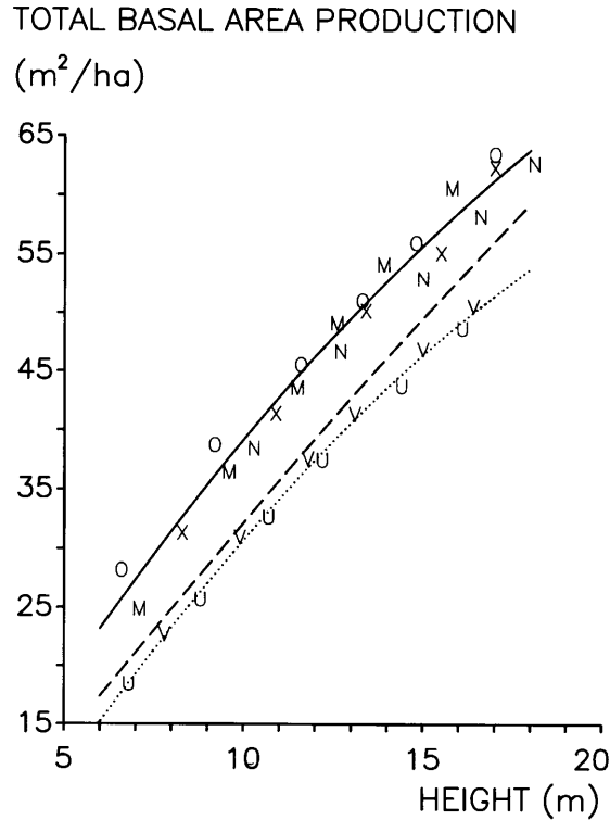
Fig. 5. Total basal area production vs. stand height for unthinned plots in the Rold (KM, KN, KO) and Grib (KU, KV, KX) areas. Regression lines are for Rold (solid), Grib (dashed), and KU + KV plots (dotted).
