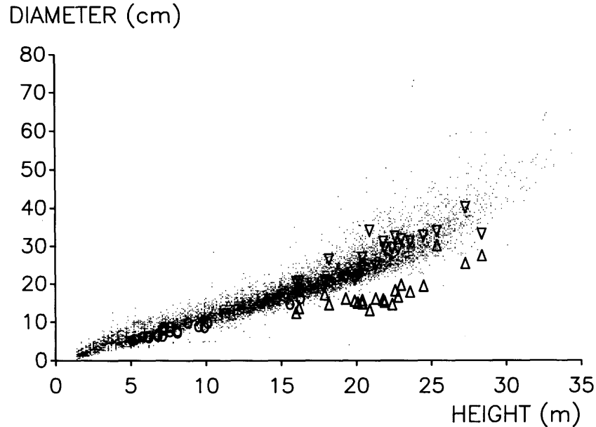
Fig. 4. Quadratic mean diameter by stand height. Symbols indicate the FMDB (•), the initial PSP (pre-treatment) (○), and the range of diameters at last PSP observation (Δ-▽).
