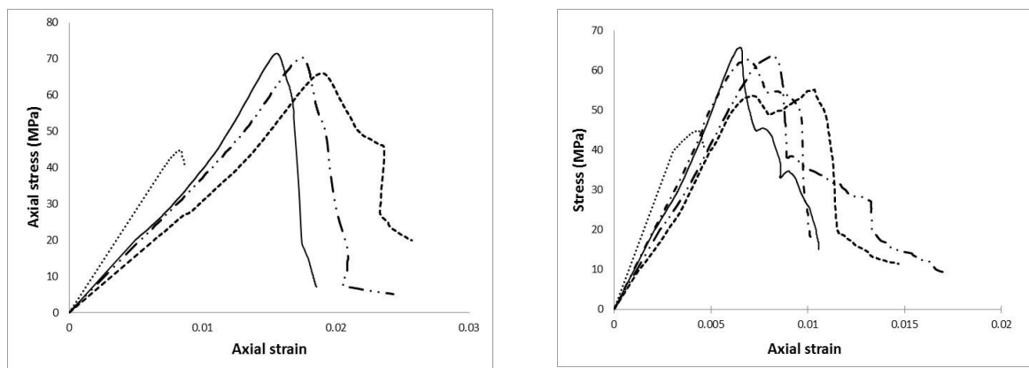
(a) 100 mm diameter and 200 mm high samples — CFRP 1 layer ..... GFRP 1 layer
