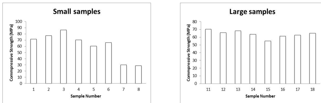
Figure 3. 28 day compressive strength for the tested samples
