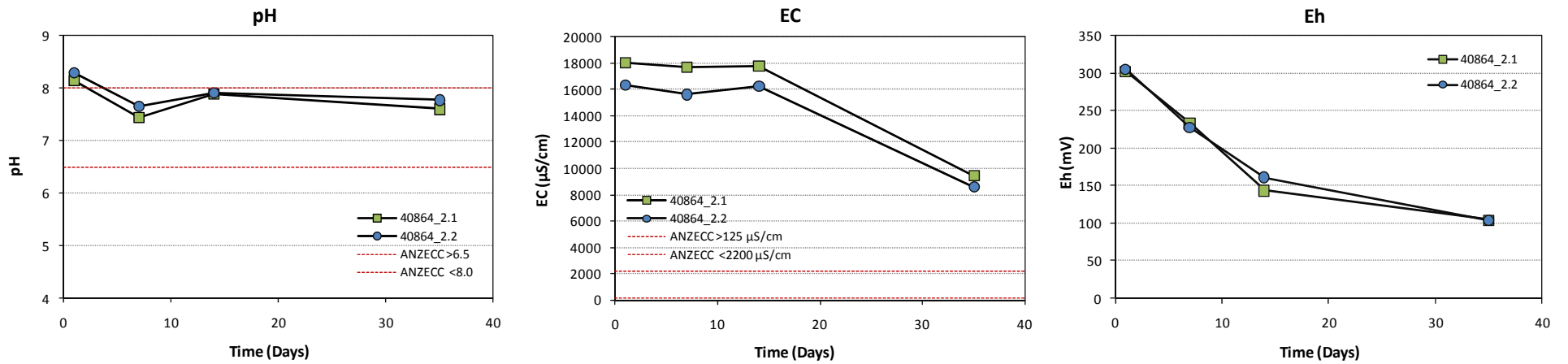
Figure 3-1: pH, EC and Eh dynamics over 35 days for the Brickworks Lagoon soil materials (40864_2.1 and 40864_2.2).
