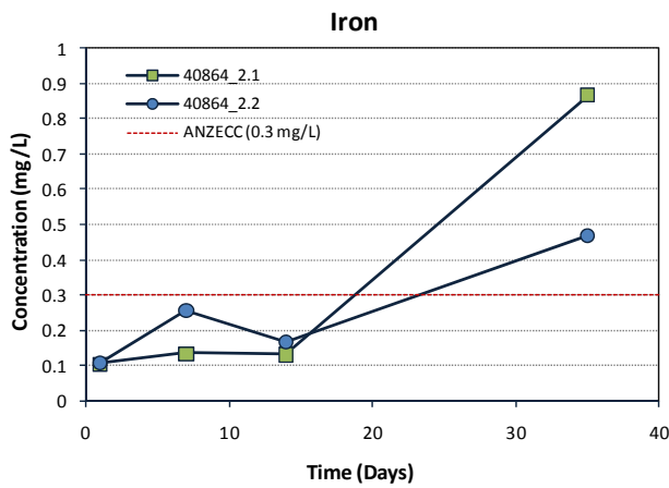
Figure 3-3: Contaminant and metalloid dynamics (Cd, Co, Cr, Cu, Fe and Mn) over 35 days for the Brickworks Lagoon soil materials (40864_2.1 and 40864_2.2).
