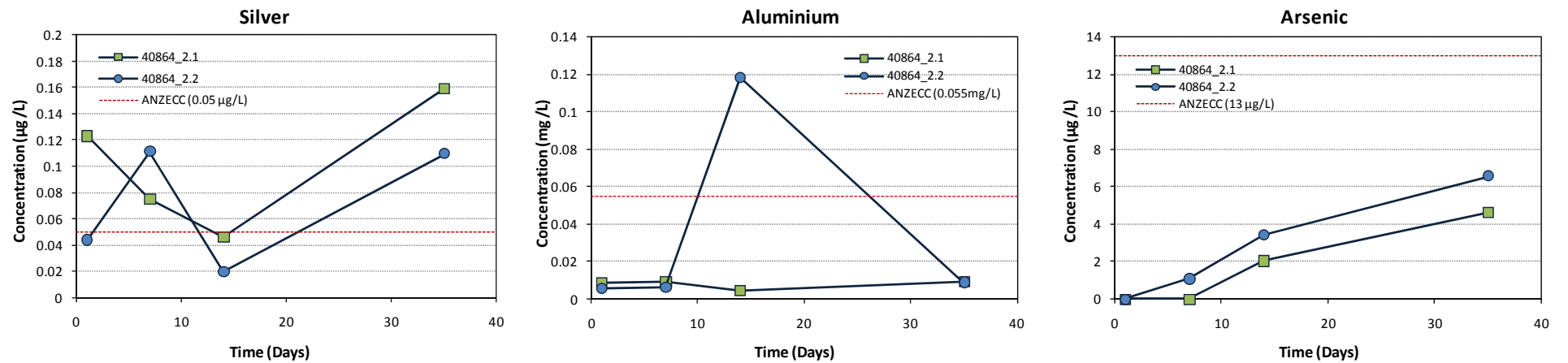
Figure 3-2: Contaminant and metalloid dynamics (Ag, Al and As) over 35 days for the Brickworks Lagoon soil materials (40864_2.1 and 40864_2.2).
