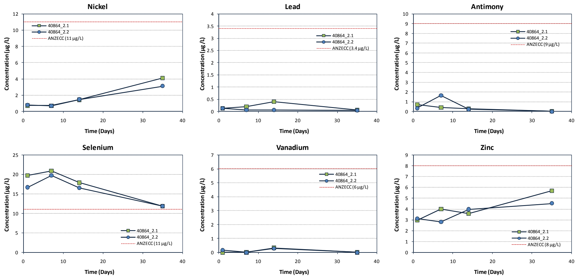
Figure 3-4: Contaminant and metalloid dynamics (Ni, Pb, Sb, Se, V and Zn) over 35 days for the Brickworks Lagoon soil materials (40864_2.1 and 40864_2.2).
