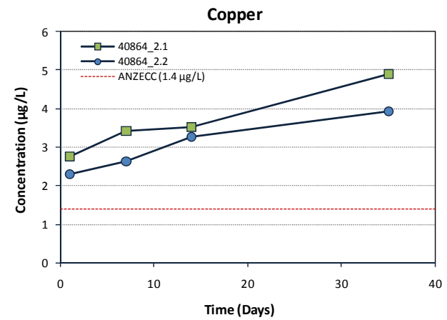
Figure 3-3: Contaminant and metalloid dynamics (Cd, Co, Cr, Cu, Fe and Mn) over 35 days for the Brickworks Lagoon soil materials (40864_2.1 and 40864_2.2).
