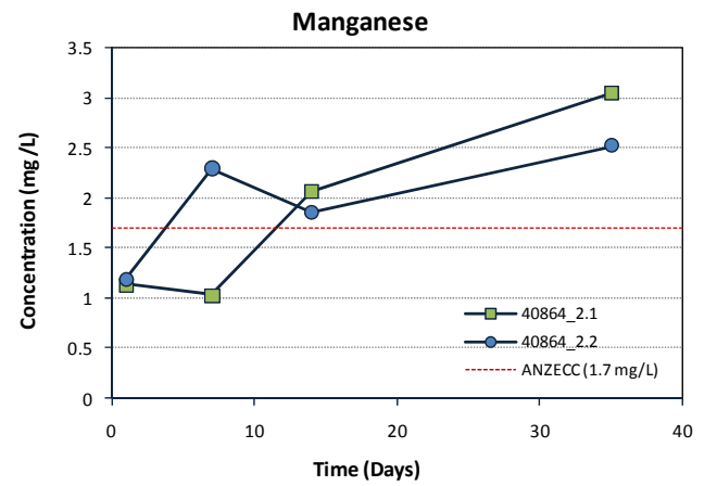
Figure 3-3: Contaminant and metalloid dynamics (Cd, Co, Cr, Cu, Fe and Mn) over 35 days for the Brickworks Lagoon soil materials (40864_2.1 and 40864_2.2).
